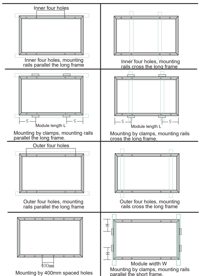
Figure 4 Installation Methods
