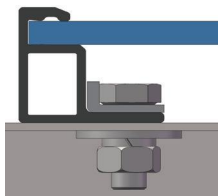
Installation with Mounting Hole Bolts:
