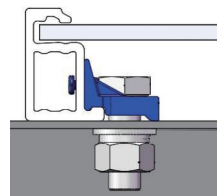
Installation with Mounting Hole Holder:
