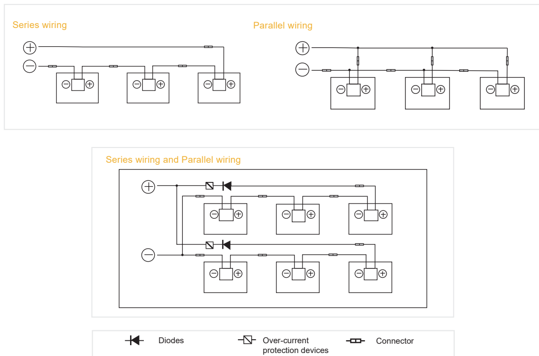
Figure 4: Electrical diagrams of series and parallel wiring
