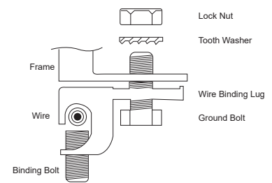
Figure 6: Installation methods
