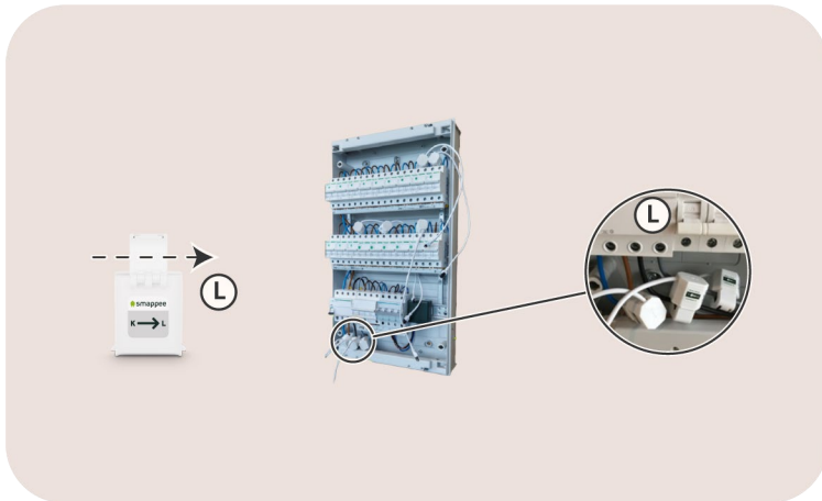
Image 5: View on the arrow on a current transformer and its installation in the distribution panel
