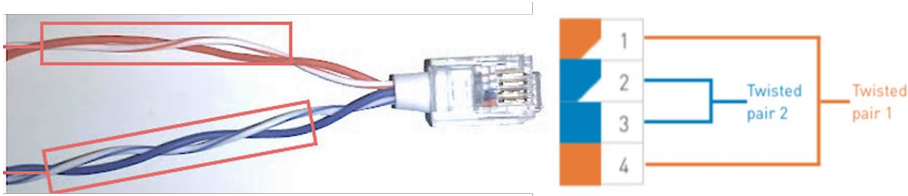
Image 17: Twisted pairs
