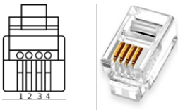
Image 18: Connector
