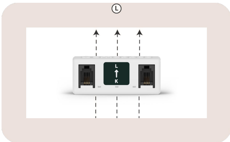
Image 7: View on the arrow on a Solid Core CT
