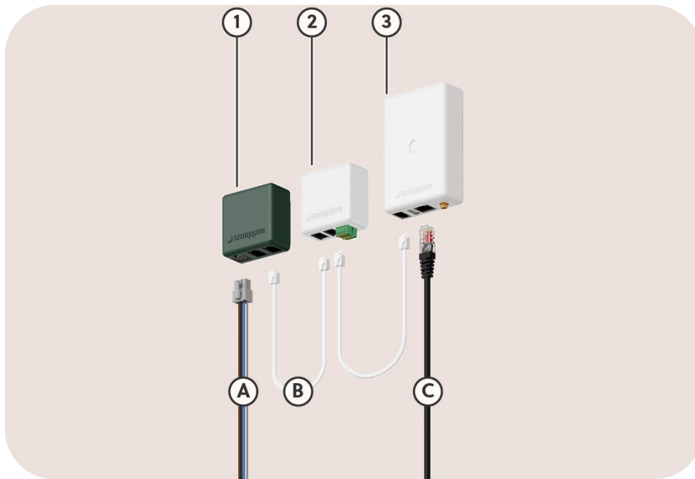
Image 12: Schematic view of the Smappee B-bus circuit
