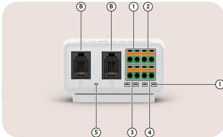
Image 11: View on an Input module
