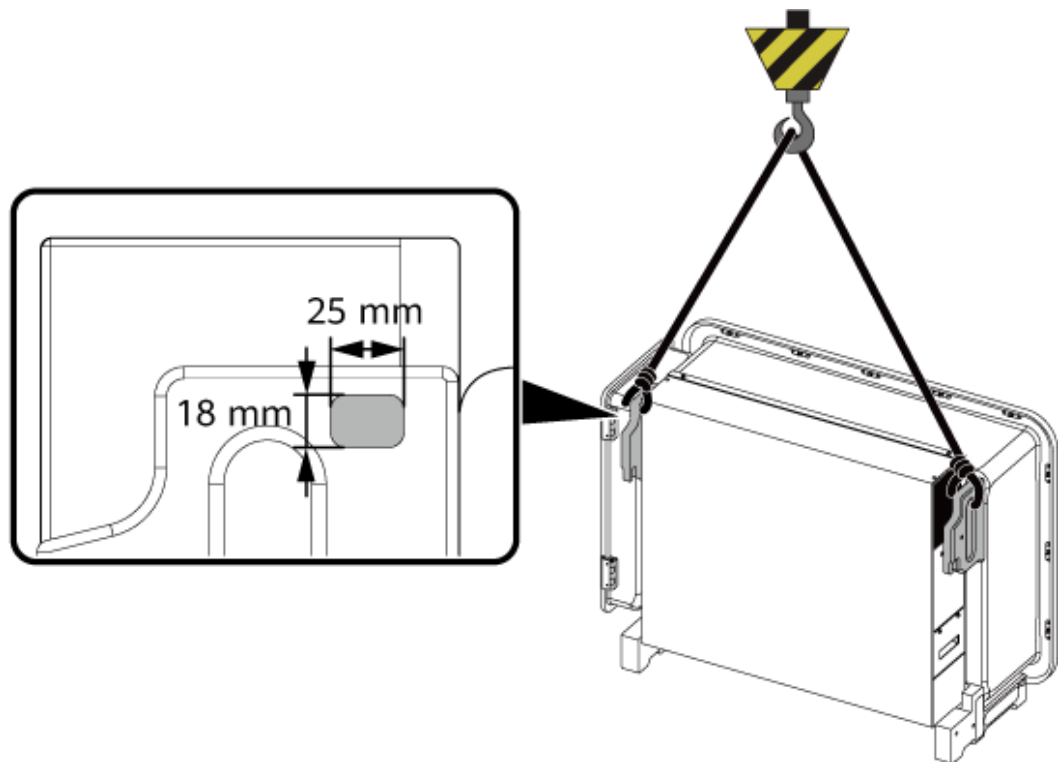
Figure 4-10 Levage
