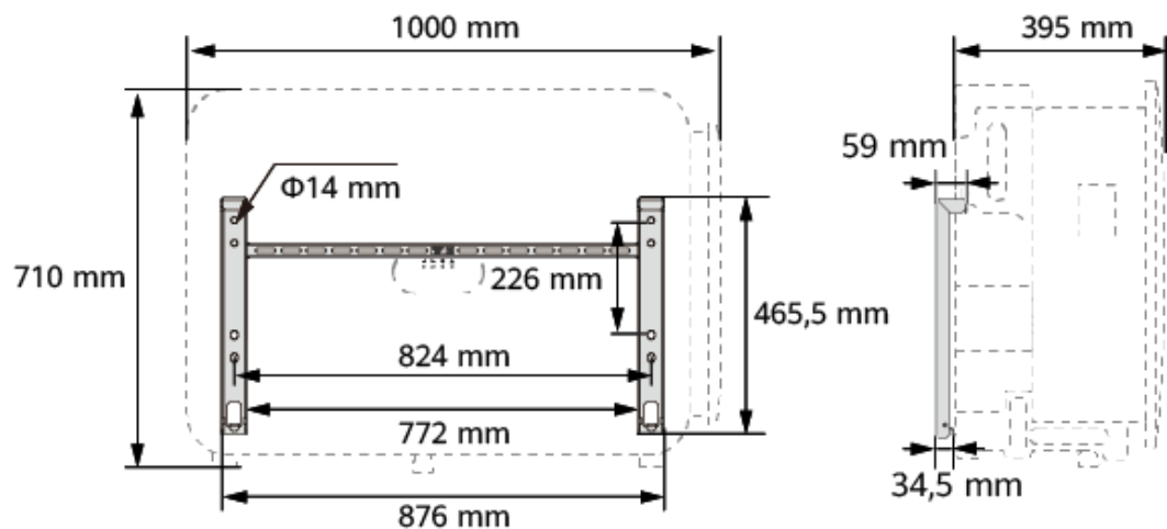
Figure 4-1 Dimensions
