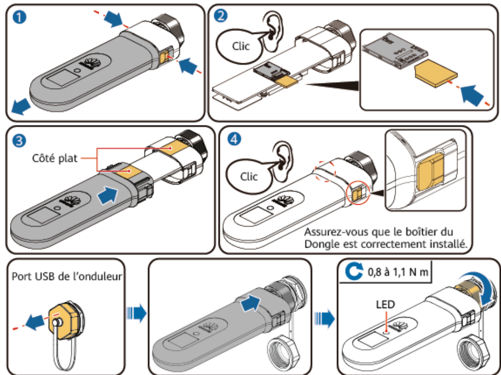
Figure 5-22 Installation du Smart Dongle 4G (SDongleB-06)
