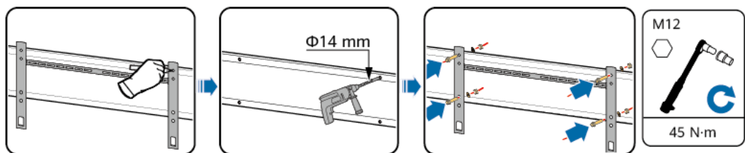
Figure 4-12 Installation du support de montage
