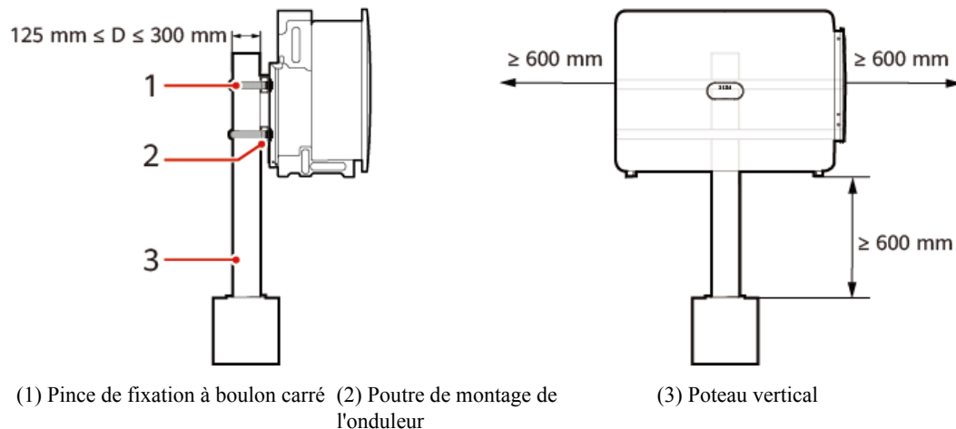
Figure 4-17 Installation de la pince de fixation
