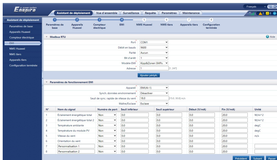
Figure 7-6 Connexion aux EMI
