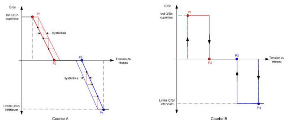
Figure 7-20 Courbe Q(U)
