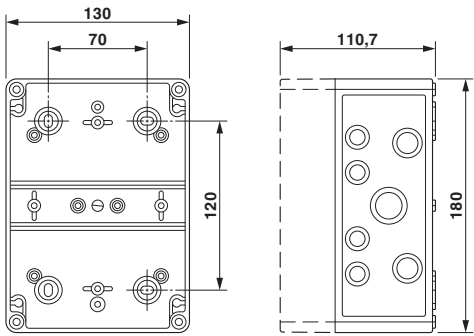
Housing dimensions
