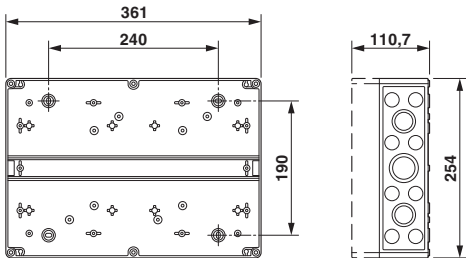
Housing dimensions
