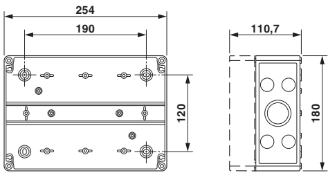
Housing dimensions
