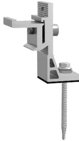
Tin Interface A with ezClick connection for ECO-Rail
