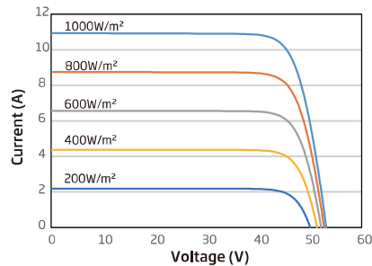
I-V CURVES OF PV MODULE (455W)
