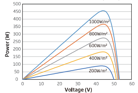
P-V CURVES OF PV MODULE (455W)
