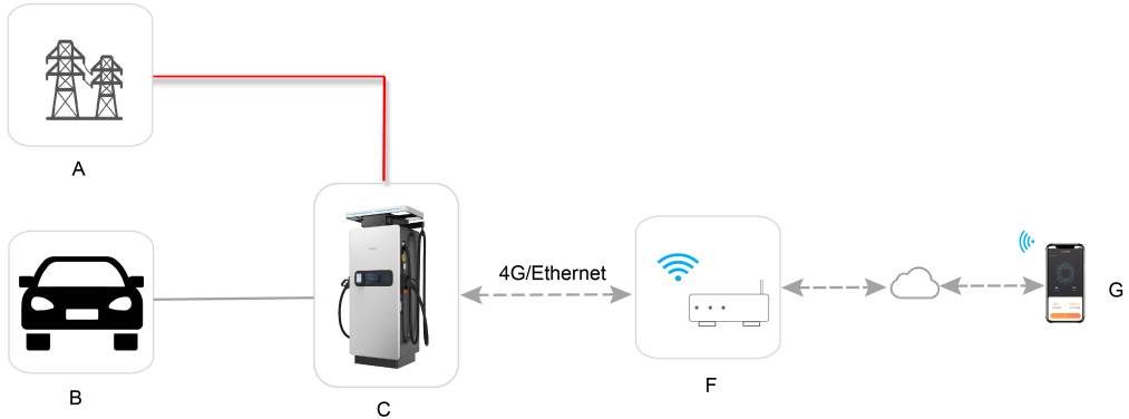
Figure 2-3 Remote Charging
