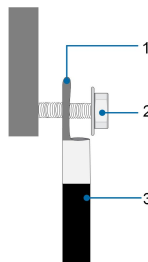
Figure 5-1 Aluminum Cable Connection
