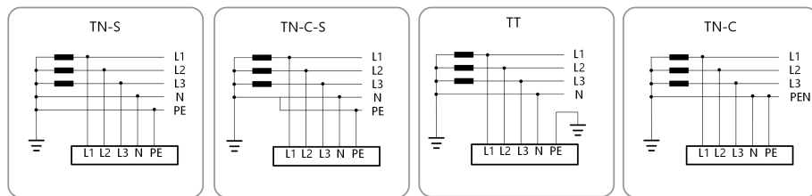
Figure 3-1 Earthing Systems
