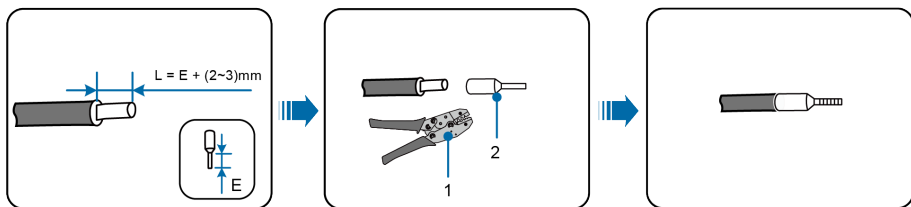
(1) Crimp tool
