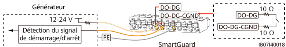
Figure E-1 Signal de Generator Control
